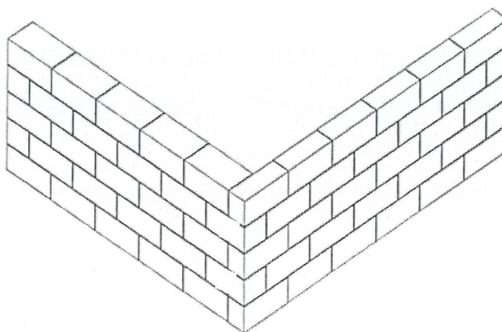
FIGURE E1: RUNNING OR STRETCHER BOND
